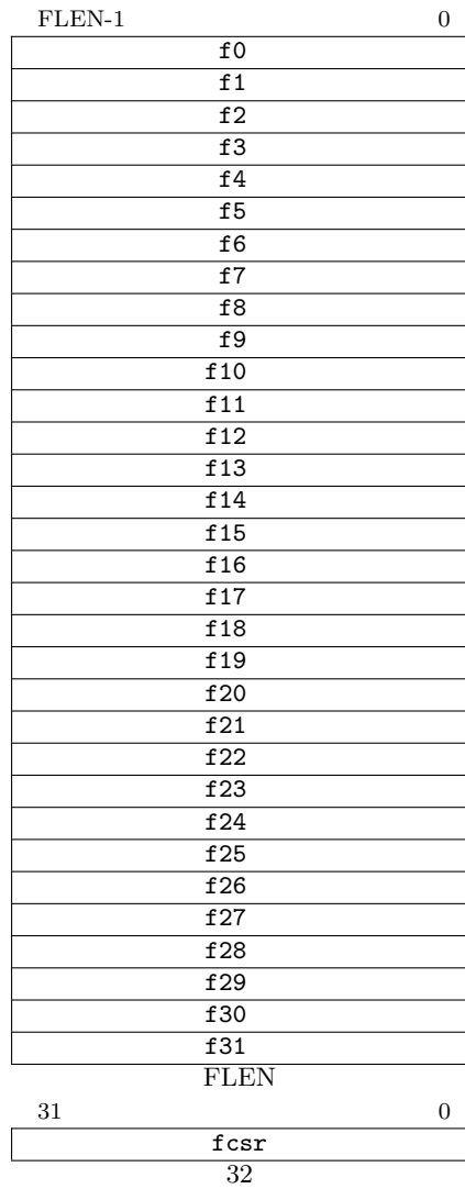
Figure 13.1: RISC-V standard F extension single-precision floating-point state.
